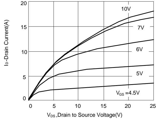
Figure 10: Output Characteristics
