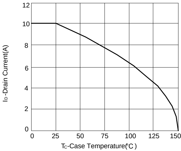
Figure 9: Continuous Drain vs Case Temperature
