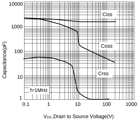
Figure 7: Capacitance vs Drain to Source Voltage
