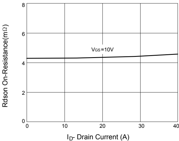
Figure 5 Rdson-drain current
