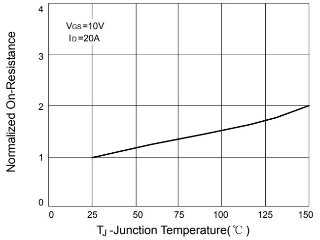
Figure 2 Rds(on)-junction temperature
