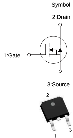
TO-252
