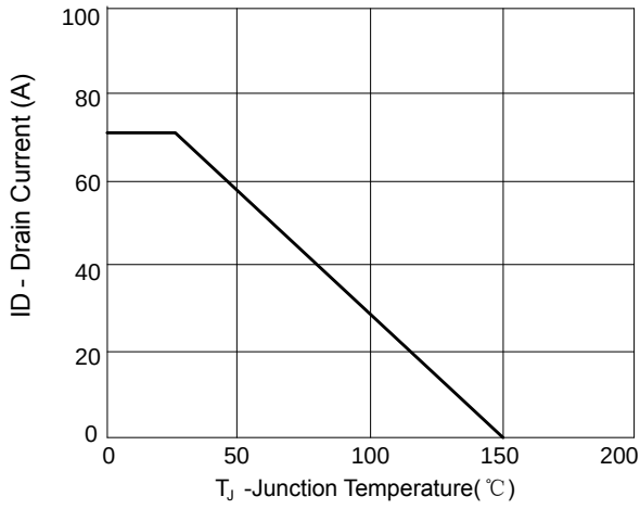
Figure 7:Power de-rating
