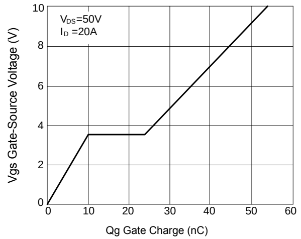
Figure 5: Gate charge
