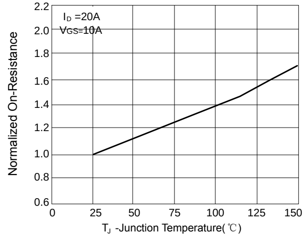
Figure 10:Rdson-junction temperature
