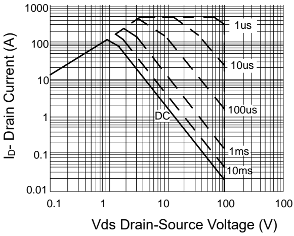
Figure 9: Output characteristics
