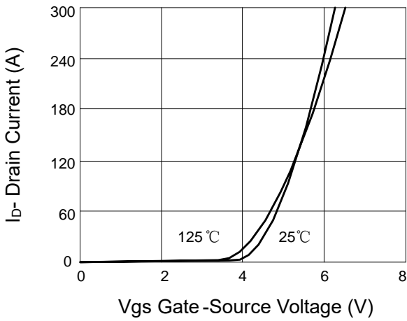
Figure 3: Transfer characteristics
