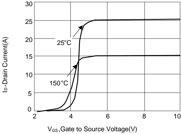
Figure 1: Transfer Characteristics
