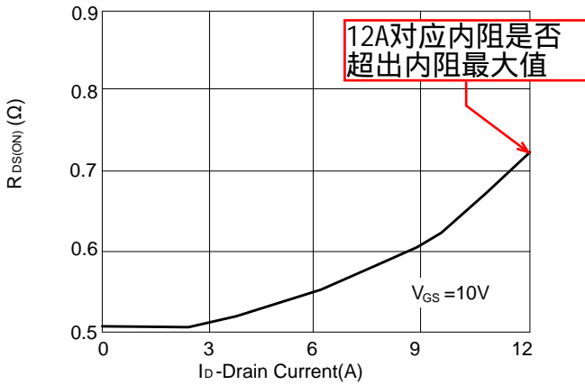
Figure 3: Drain to Source On-Resistance vs Drain Current
