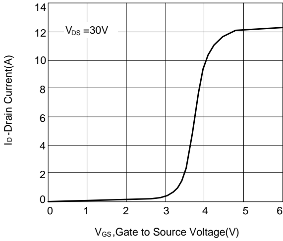
Figure 1: Transfer Characteristics
