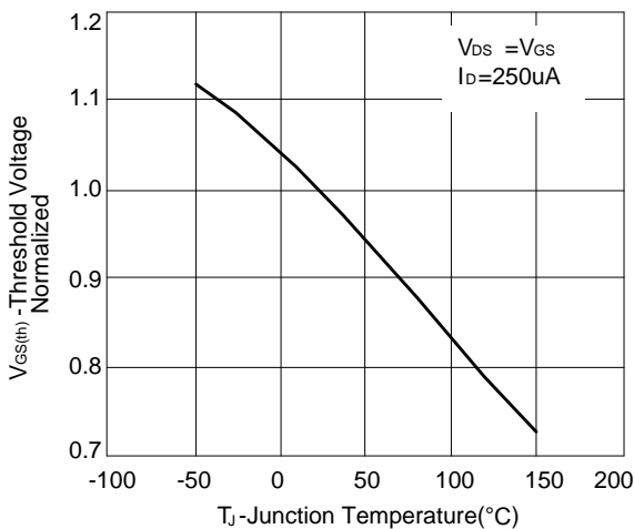
Figure 5: Threshold Voltage vs Junction Temperature
