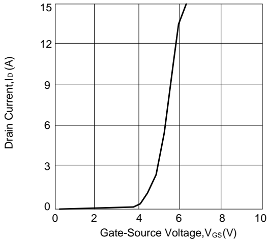
Figure 9: Drain Current vs. Gate-Source Voltage
