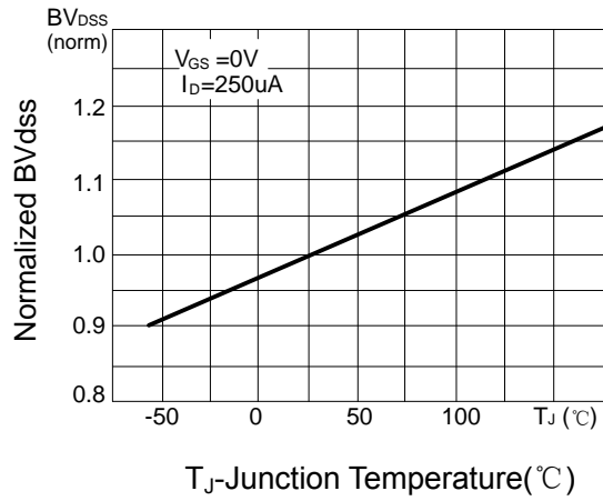
Tj-Junction Temperature(°C) Figure 8: BVdss vs junction temperature
