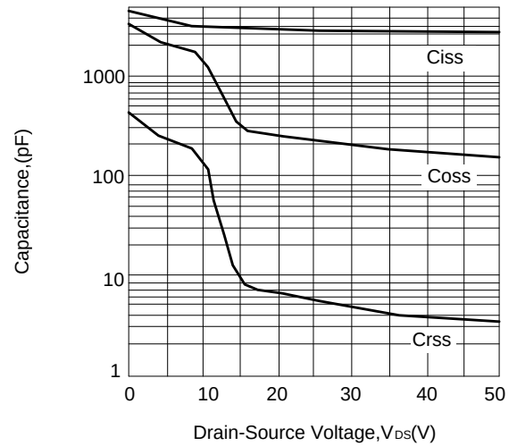
Figure 4: Capacitance Characteristics
