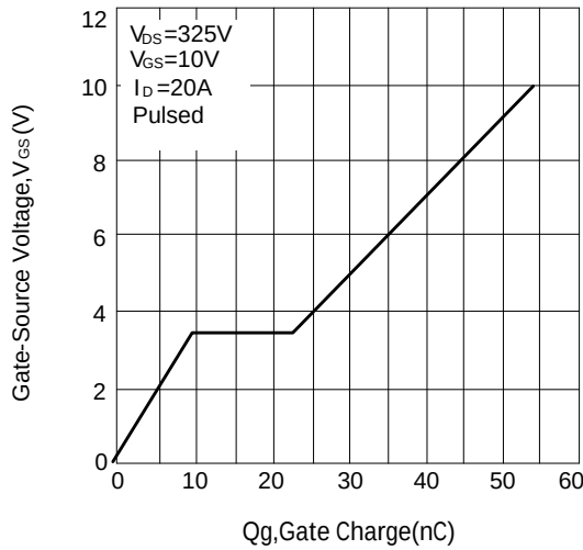
Figure 3: Gate Charge vs. Gate to Source Voltage
