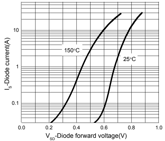
Figure 8. Body-Diode Characteristics
