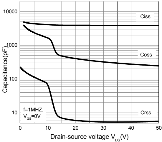
Figure 9. Capacitance Characteristics
