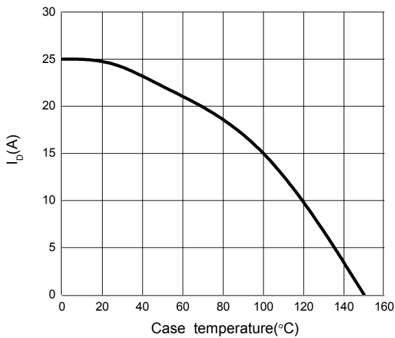
Figure 11. Continuous Drain Current vs. Temperature
