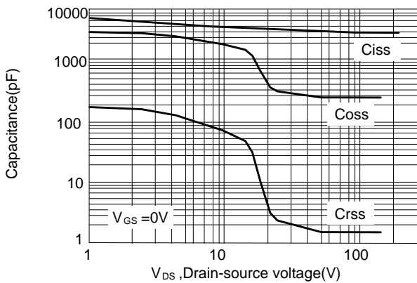
Figure 5: Capacitance characteristics
