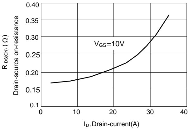
Figure 3: Drain to Source On-resistance Drain Current
