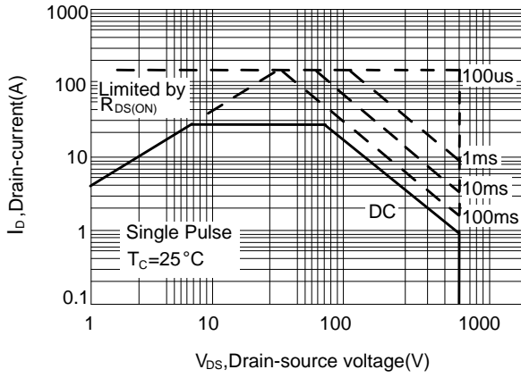
Figure 9: Maximum safe operation area
