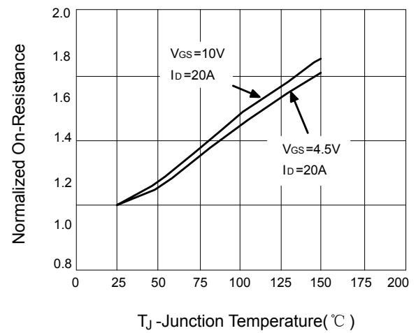
Figure 4 Rdson-junction temperature
