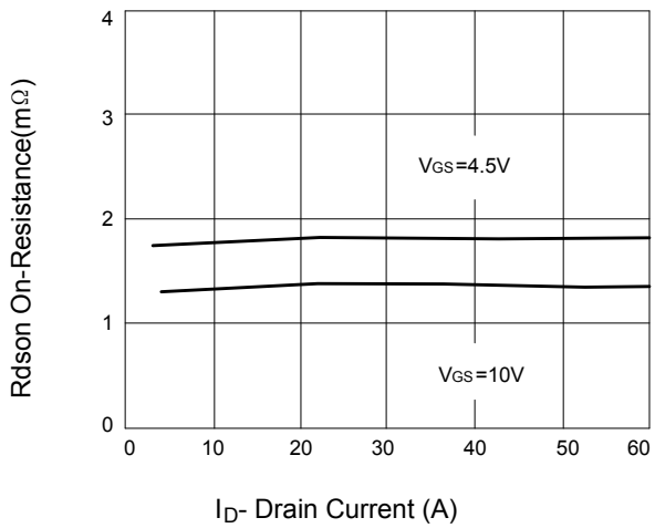
Figure 3 Rdson-drain current
