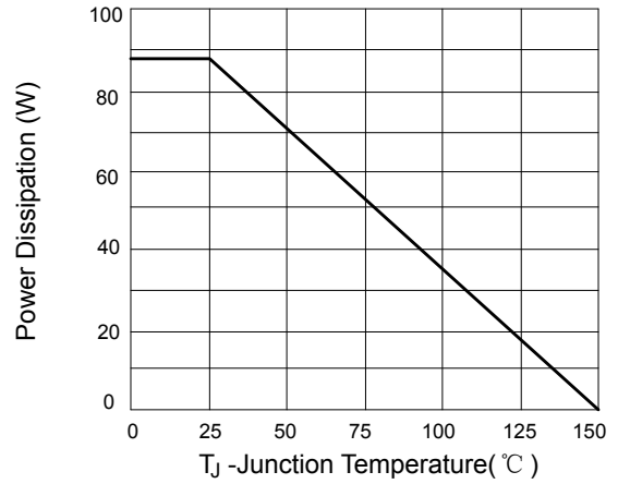
Figure 8 Power de-rating
