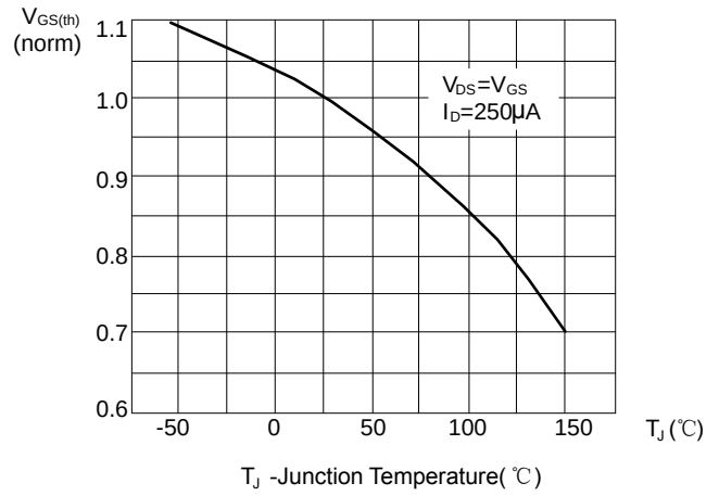
Figure 10: Vgs vs junction temperature
