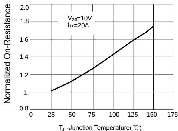
Figure 4: Rdson-temperature
