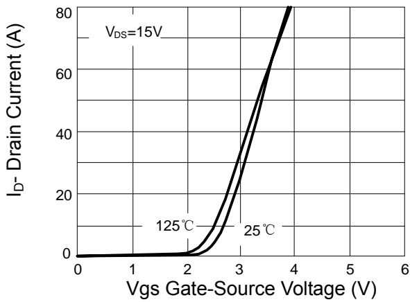
Vgs Gate-Source Voltage (V) Figure 3: Transfer characteristics
