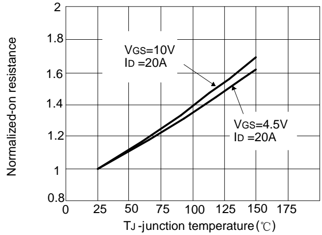
Figure.2 Rds(on)-junction temperature
