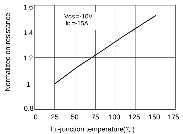
Fig.6 drain-source on-resistance
