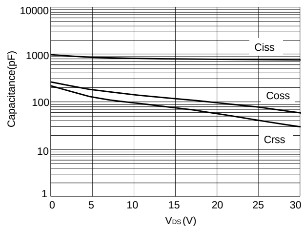
Figure 6: Capacitance Characteristics
