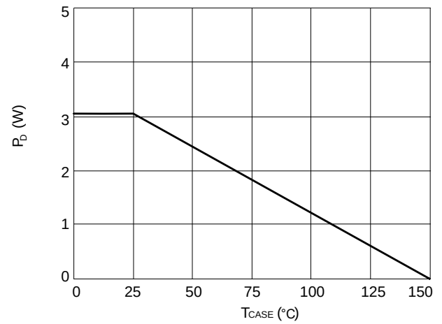
Figure 8: Power De-rating
