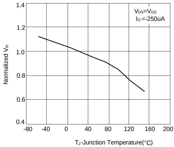
Figure 9: Normalized Threshold Voltage vs. Junction Temperature
