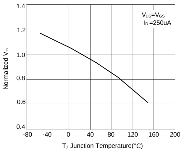
Figure 9: Normalized Threshold Voltage vs. Junction Temperature
