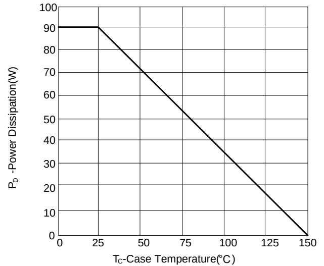
Figure 11: Power Dissipation vs Case Temperature
