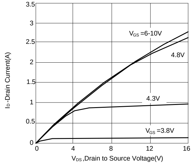
Figure 10: Output Characteristics
