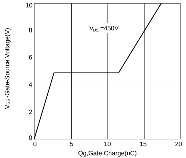
Figure 8: Gate Charge vs Gate to Source Voltage
