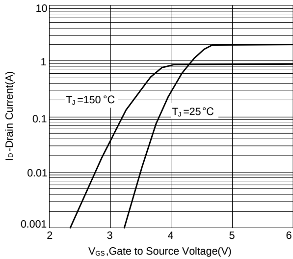
Figure 1: Transfer Characteristics
