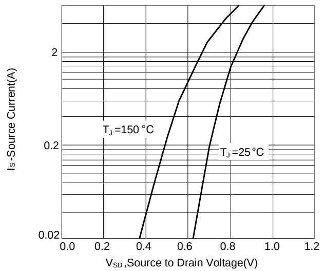
Figure 2: Body Diode Characteristics
