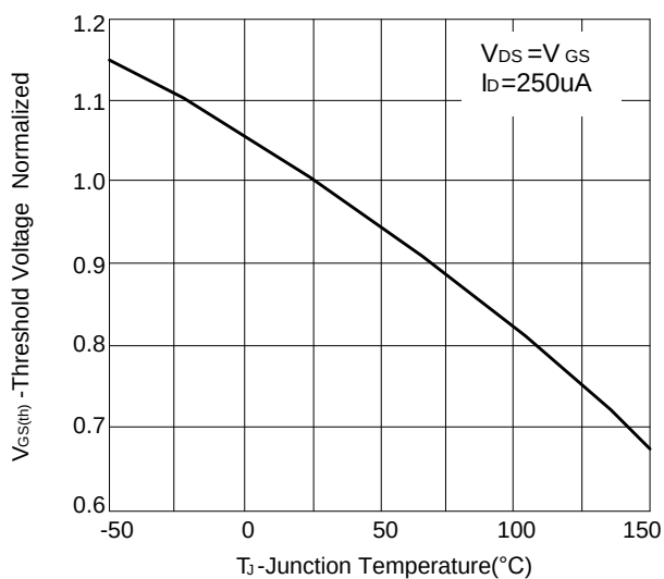
Figure 5: Threshold Voltage vs Junction Temperature
