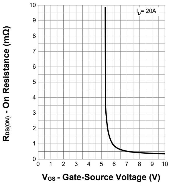
On-resistance gate source voltage
