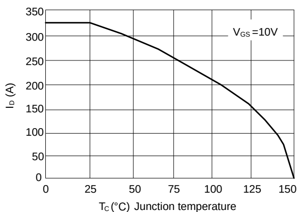
Figure 10: Current de-rating
