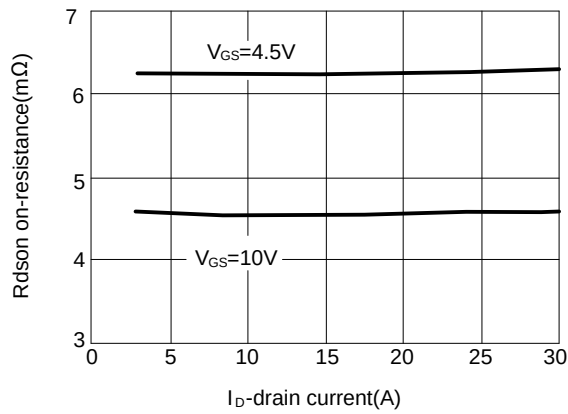
Figure 5 :Rdson-drain current
