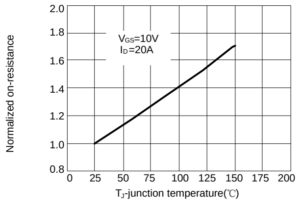
Figure 2 :Rdson-junction temperature
