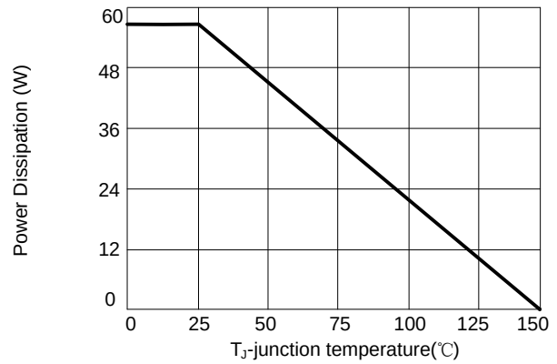
Figure 8 :Power de-rating
