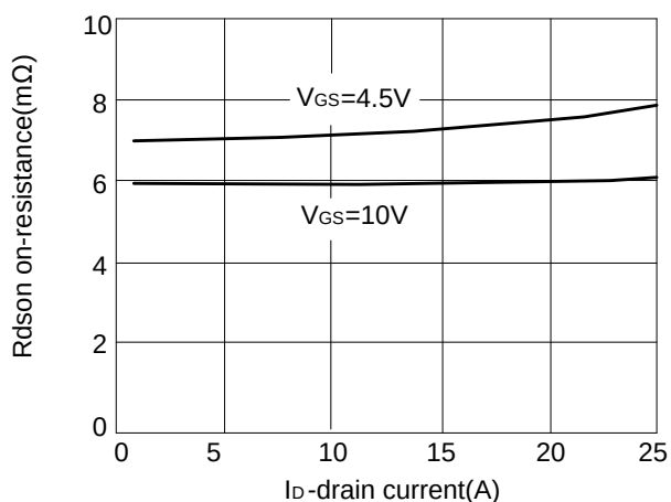
Figure 5: Rdson-drain current
