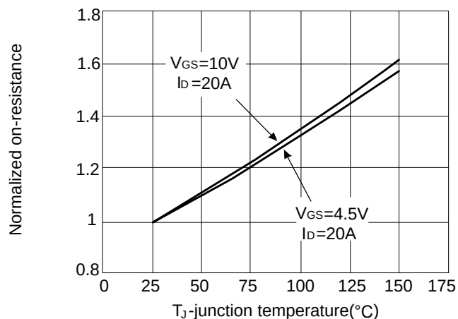
Figure 4: Rdson-junction temperature
