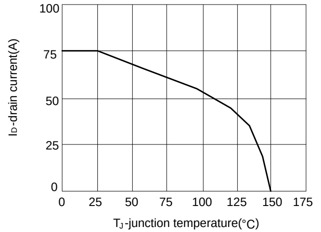
Figure 10: Current de-rating
