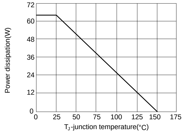
Figure 8: Power de-rating
