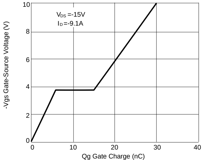
Figure 4: Gate Charge
