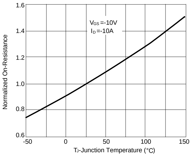
Figure 5: Drain-Source On-Resistance
