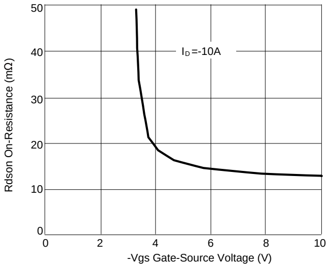
Figure 3: Rds(on) vs. Vgs
