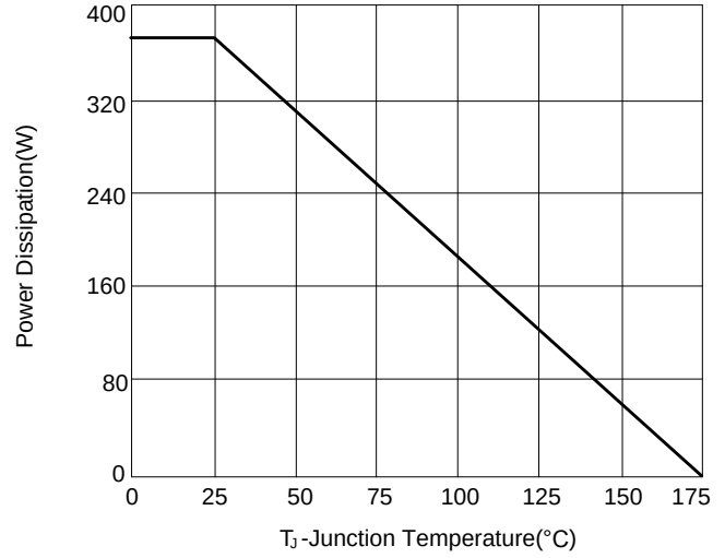
Figure 8: Power De-rating
