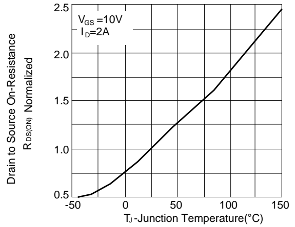
Figure 4: Drain to Source On-Resistance vs Junction Temperature
