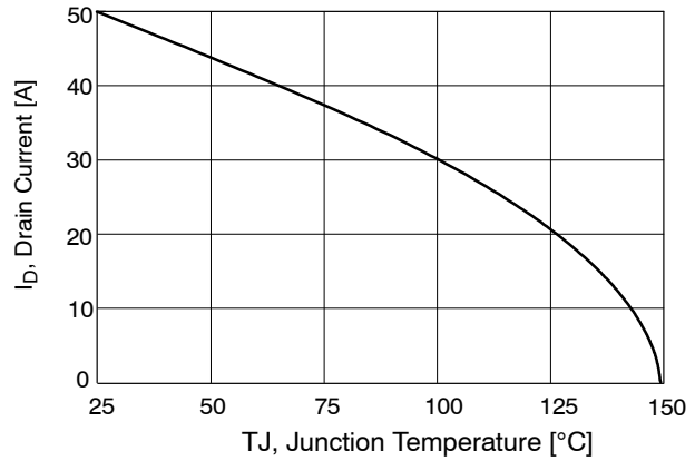
Figure10:Maximum drain current vs Junction temperature
