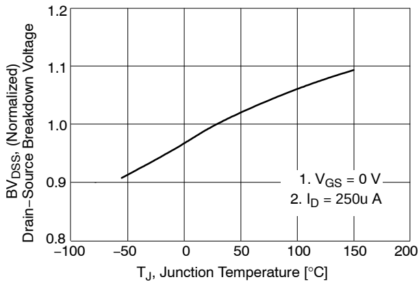
Figure7:Breakdown voltage variation vs Junction temperature
