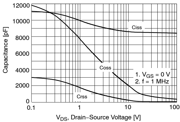
Figure5:capacitance characteristics
