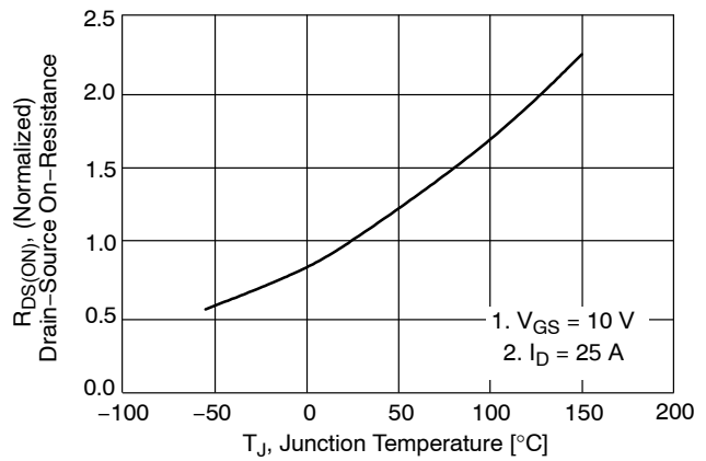
Figure8:On-resistance variation vs Junction temperature
