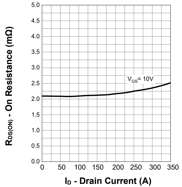
On Resistance
