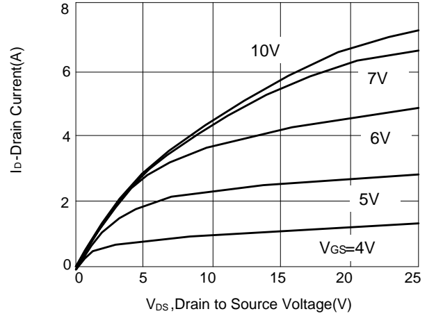
Figure 10: Output Characteristics
