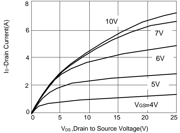
Figure 10: Output Characteristics
