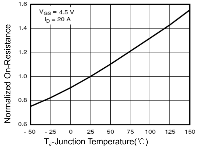
Figure 2 Rdson-Junction Temperature
