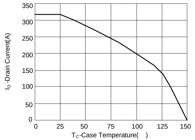
Figure 10: Current De-rating
