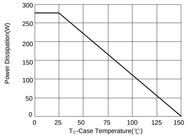
Figure 8: Case De-rating
