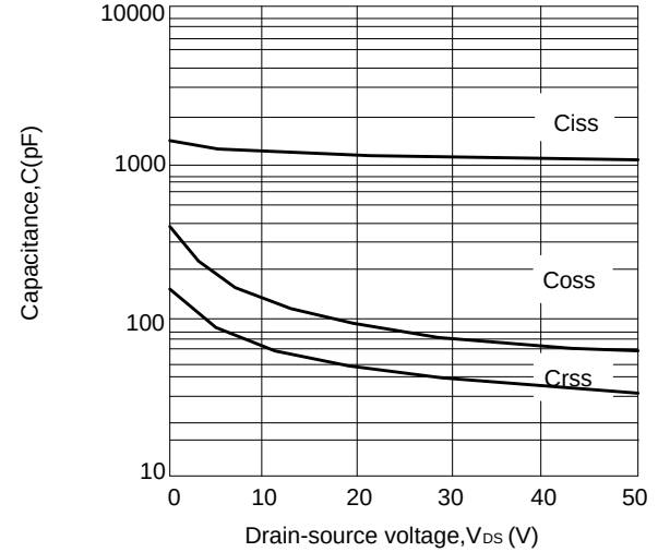
Figure 4: Capacitance characteristics
