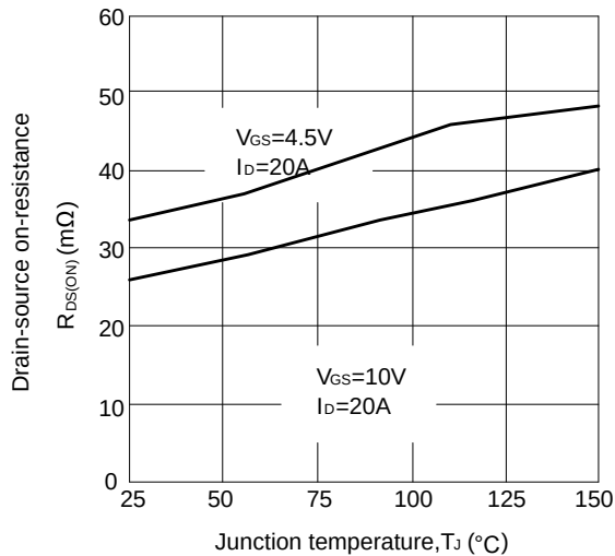
Figure 5: Drain-source on-resistance vs. junction temperature
