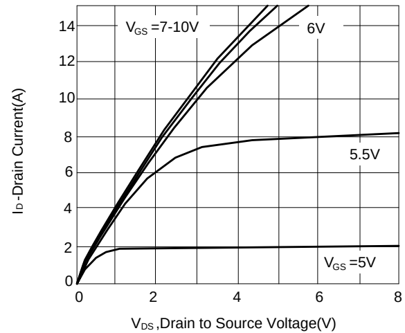
Figure 10: Output Characteristics
