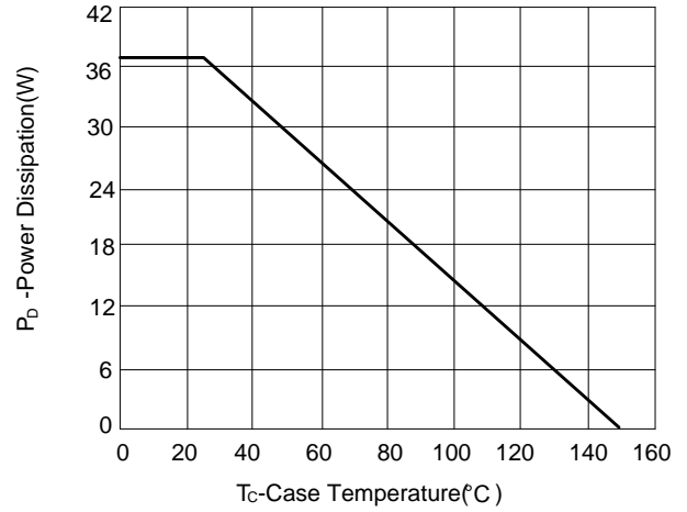
Figure 10: Power Dissipation vs Case Temperature
