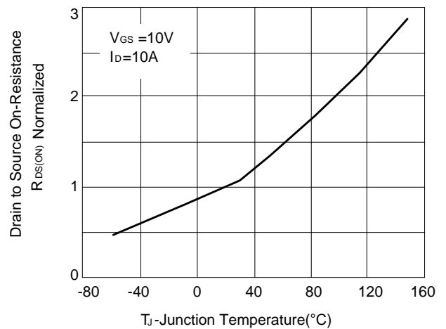
Figure 6: Drain to Source On-Resistance vs Junction Temperature
