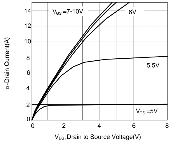
Figure 10: Output Characteristics
