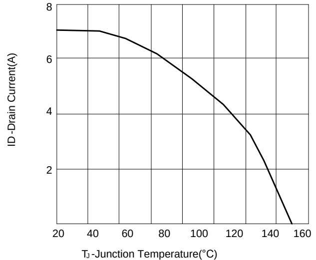
Figure 10: Continuous Drain vs Junction Temperature
