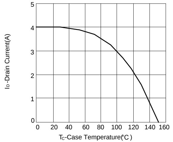
Figure 10: Continuous Drain vs Case Temperature
