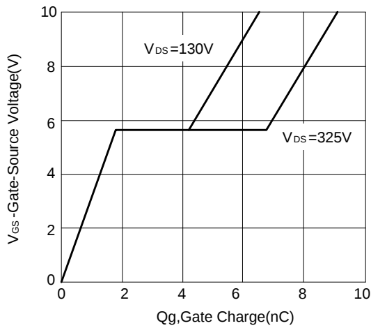
Figure 9: Gate Charge vs Gate to Source Voltage
