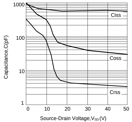
Figure 4: Capacitance Characteristics
