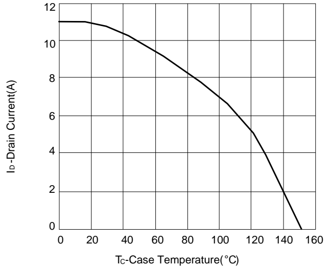
Figure 10: Drain Current Derating
