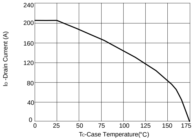
Figure 9: Current De-rating
