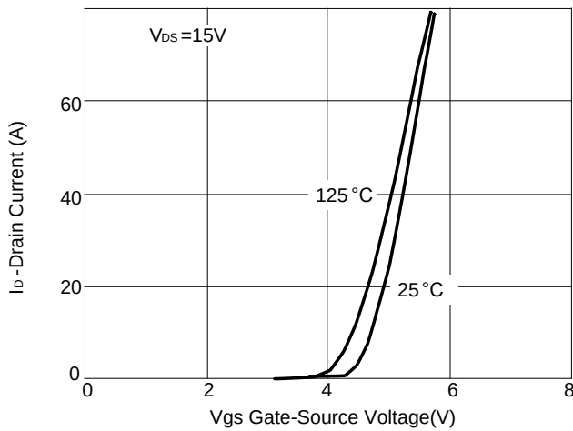
Figure 3: Transfer Characteristics
