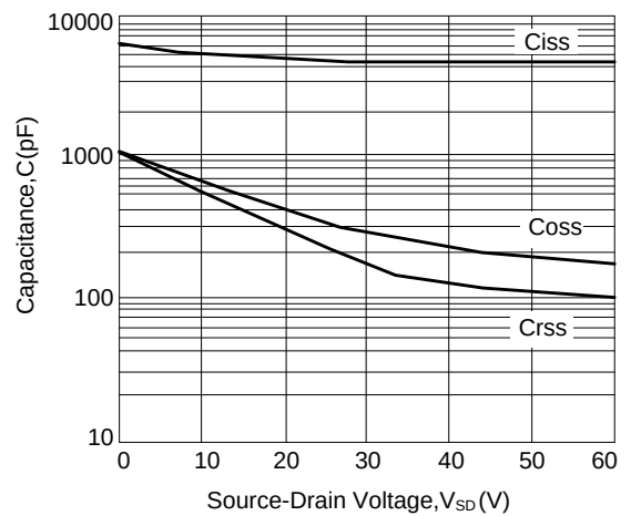
Figure 4: Capacitance Characteristics
