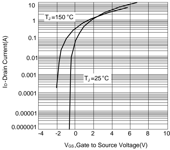
Figure 1: Transfer Characteristics
