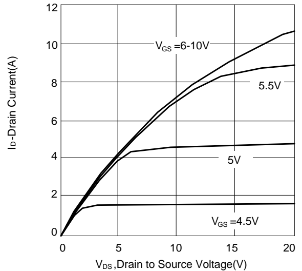
Figure 10: Output Characteristics
