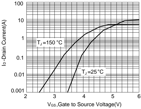
Figure 1: Transfer Characteristics
