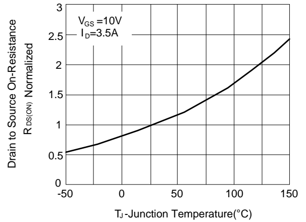
Figure 4: Drain to Source On-Resistance vs Junction Temperature
