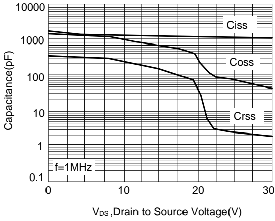
Figure 7: Capacitance vs Drain to Source Voltage
