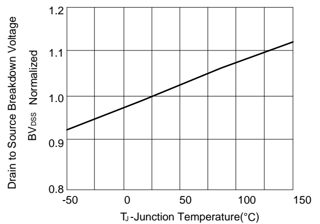
Figure 6: Breakdown Voltage vs Junction Temperature
