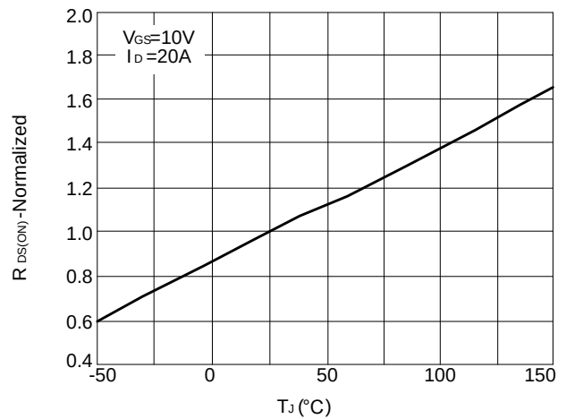
Figure 4: Rds(on) vs. Temperature
