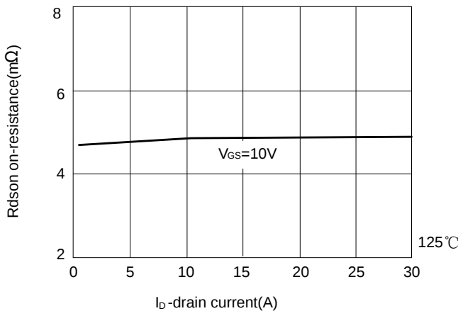
Figure 5: R_{DS(on)} -drain current
